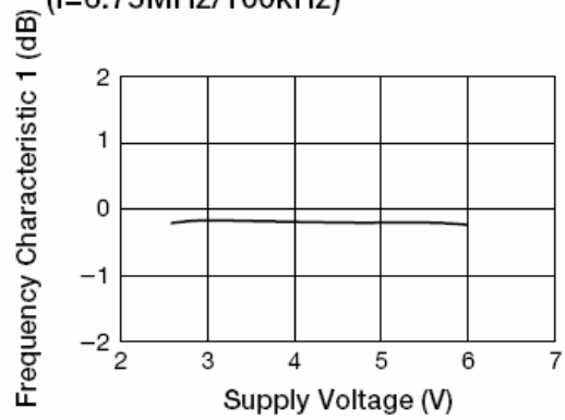
Frequency Characteristic 1 vs Supply Voltage (f=6.75MHz/100kHz)
