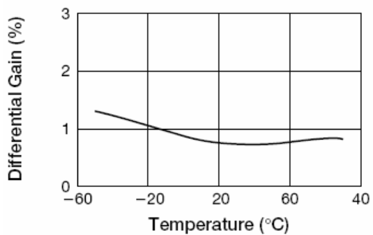
Differential Gain vs Temperature
