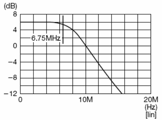
Frequency Characteristic [lin]
